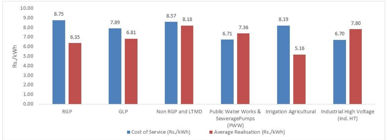
Figure 2: Category-wise cost of service and average realisation of MGVCL (Rs./kWh)
